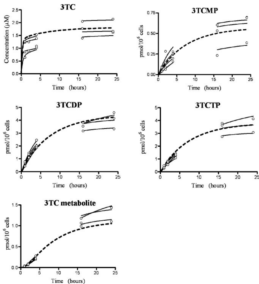
FIG. 3. Ex vivo population (dashed line) and individual (solid line) predictions and measured data (○) (5 \mu\text{M} experiments).
